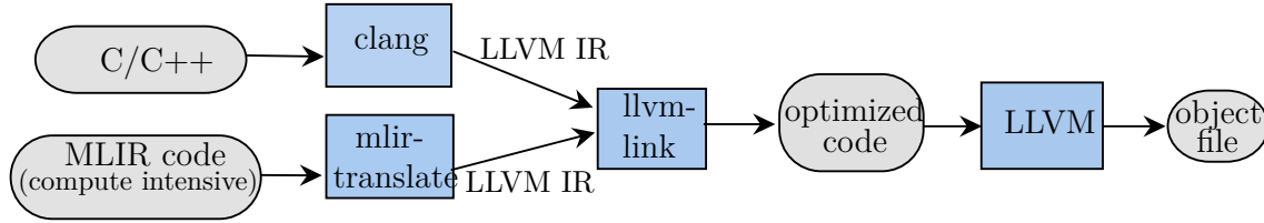
Figure 3.2: Generalized compilation view of MLIR and C/C++ code
