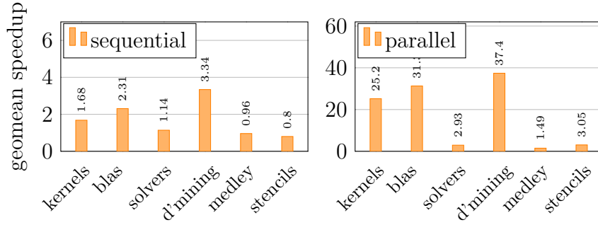
Figure 5.8: Geomean speedups of ROSE/PolyOpt compared to the baseline ROSE compiler
