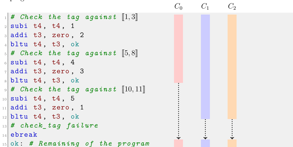
Figure 4.1 – Example of check_sandbox ( t4 , \{1,2,3,5,6,7,8,10,11\} ) and the resulting path analysis in three contexts: C_0 ( tag = 7 ), C_1 ( tag ∈ {1,10} ) and C_2 ( tag ∈ {1, 2, 3, 5, 6, 7, 8, 10, 11} )
