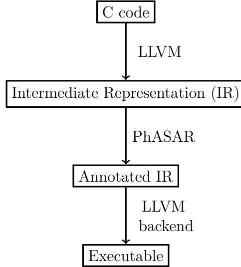
Figure 3.10 – DFI instrumentation workflow
