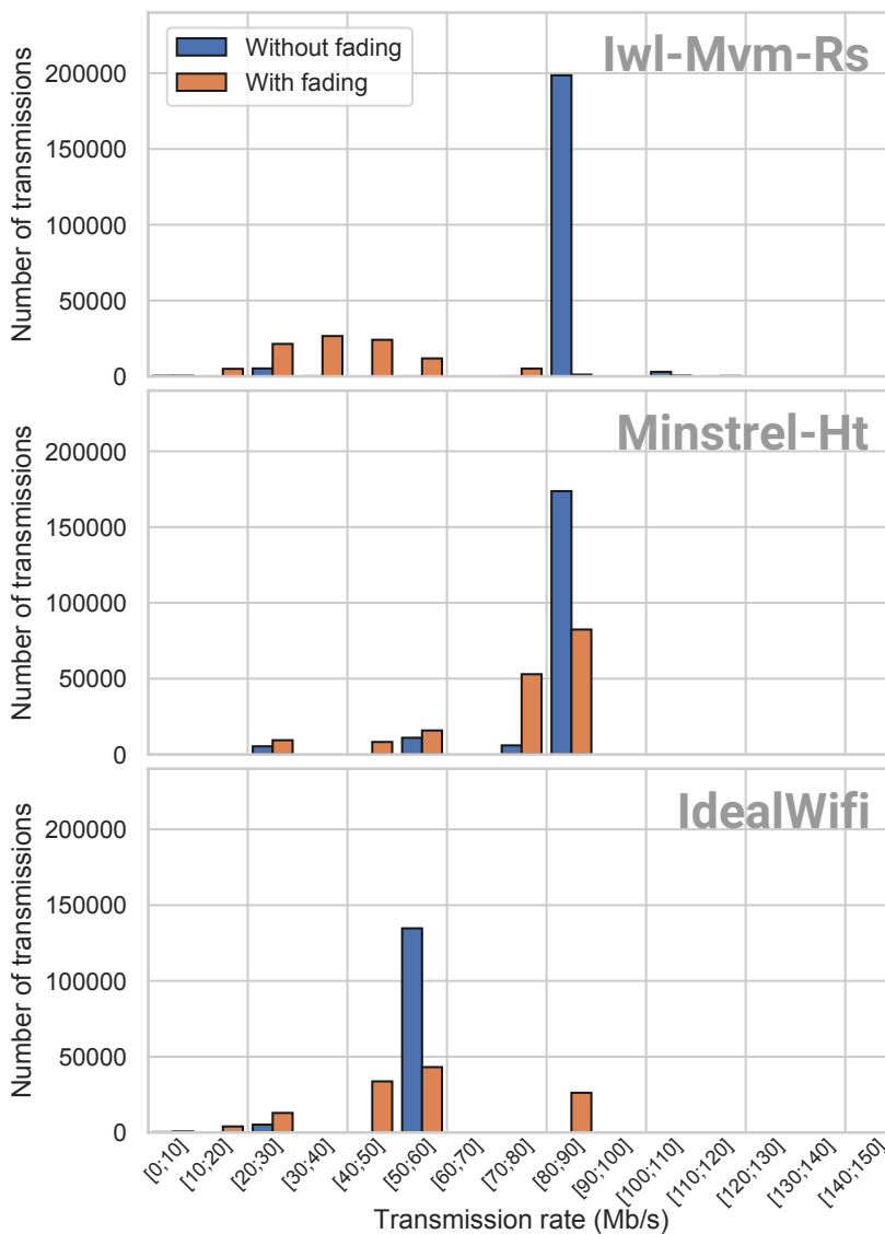
Figure 5.8: Scenario #1: Distribution of the used transmission rates for the frame sent by the source, without or with fading and for a distance of 45 m. Top to bottom: IWL-MVM-Rs, MINSTREL-HT, IDEALWIFI.
