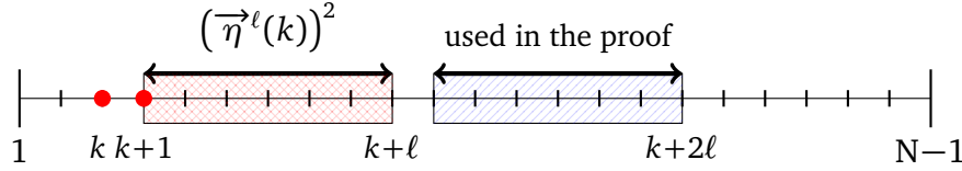
Figure 3.9: Replacement for the local function \overline{\eta}(k)\overline{\eta}(k+1) when k + 2\ell \leq N - 1 .
