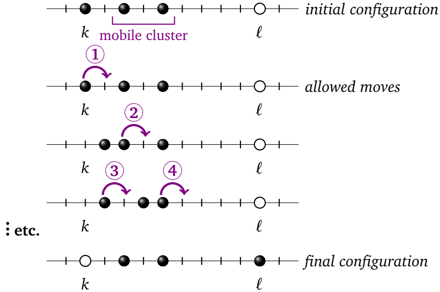
Figure 3.5: Illustration of allowed moves using the mobile cluster, in order to exchange \eta(k) with \eta(\ell) .
