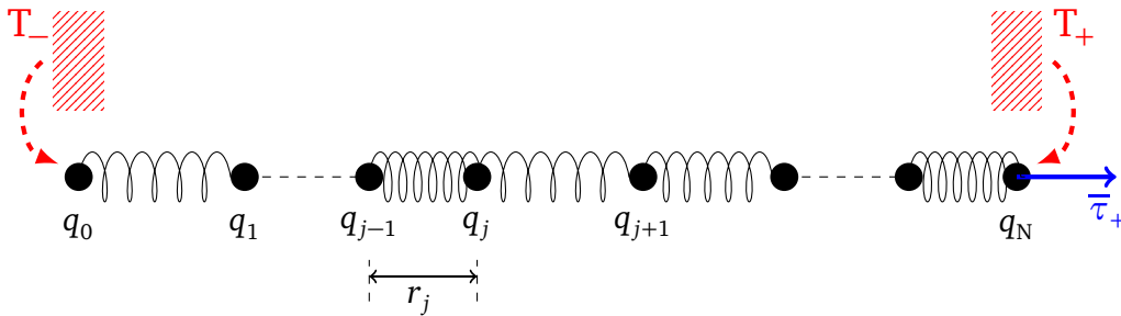
Figure 2.2: Oscillator chains with heat baths and one boundary force.
