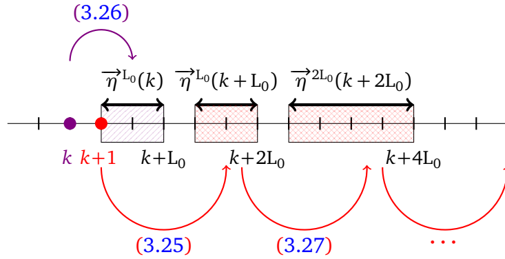
Figure 3.2: Illustration of steps (3.25)–(3.27).
