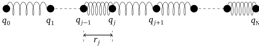
Figure 2.1: One-dimensional coupled oscillators.
