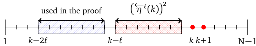
Figure 3.10: Replacement for the local function \overline{\eta}(k)\overline{\eta}(k+1) when k + 2\ell > N - 1 .
