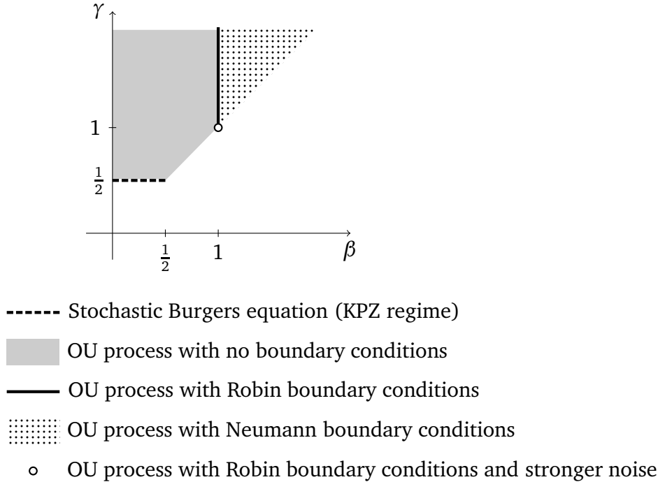
Figure 3.7: Macroscopic density fluctuations. In the region \beta > \gamma the process is not defined (negative rates). OU stands for Ornstein-Uhlenbeck.
