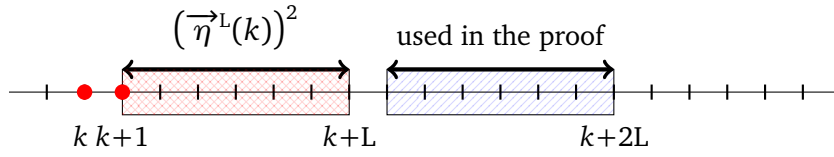
Figure 3.1: Replacement for the local function \bar{\eta}(k)\bar{\eta}(k+1) .
