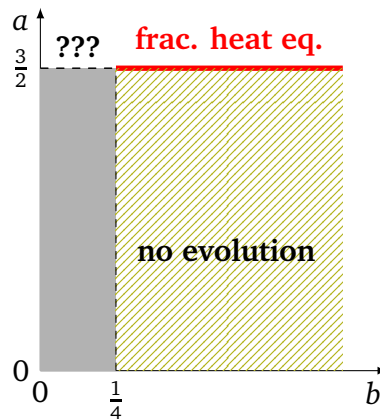
Figure 2.4: ENERGY FLUCTUATIONS: value of the time scale exponent a as a function of the anharmonicity exponent b .
