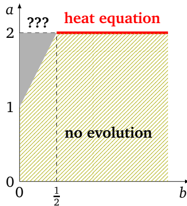
Figure 2.3: VOLUME FLUCTUATIONS: value of the time scale exponent a as a function of the anharmonicity exponent b .
