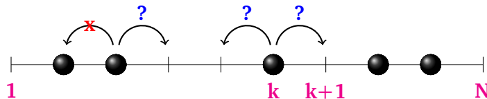
Figure 1.1: One-dimensional exclusion process with N sites ( N \in \mathbb{N} being the scaling parameter).
