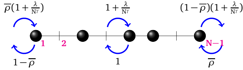
Figure 3.8: Illustration of the jump rates. The leftmost and rightmost rates are the entrance/exiting rates.
