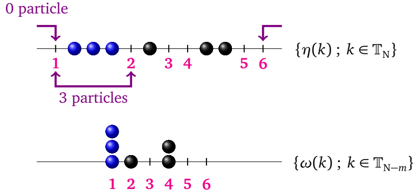
Figure 4.4: TOP: configuration in the exclusion dynamics. BOTTOM: the associated zero-range configuration.
