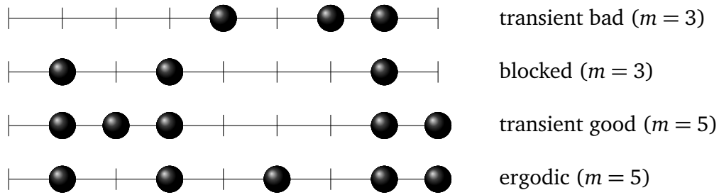
Figure 4.3: Four examples of configurations which belong to the different classes ( N = 9 ).
