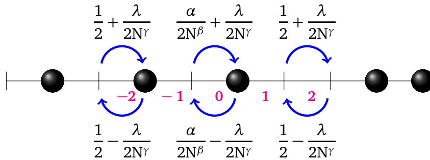
Figure 3.6: Illustration of the jump rates. The bond of vertices \{-1, 0\} has particular rates.
