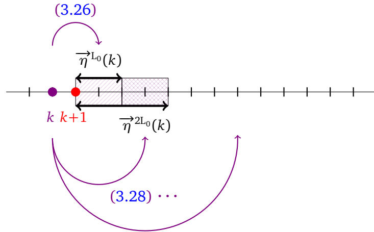
Figure 3.3: Illustration of step (3.28): successive replacements.
