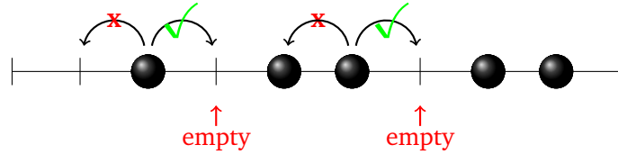
Figure 3.4: Allowed jumps are denoted by ✓. Forbidden jumps are denoted by x.
