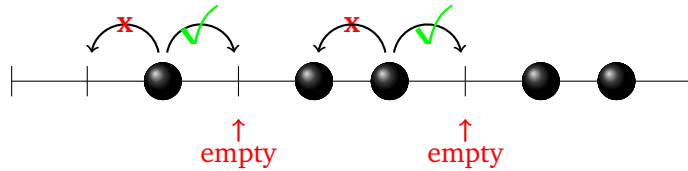
Figure 4.1: Allowed jumps are denoted by ✓. Forbidden jumps are denoted by x.
