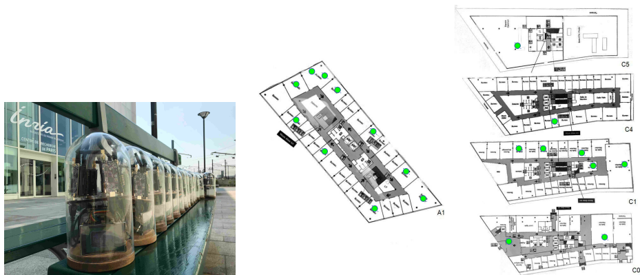
(a) The Inria-Paris Open-TestBed before deployment. 20 domes contain a total of 80 OpenMote B boards. (b) Location of the OpenTestBed domes within Inria-Paris buildings A and C.
