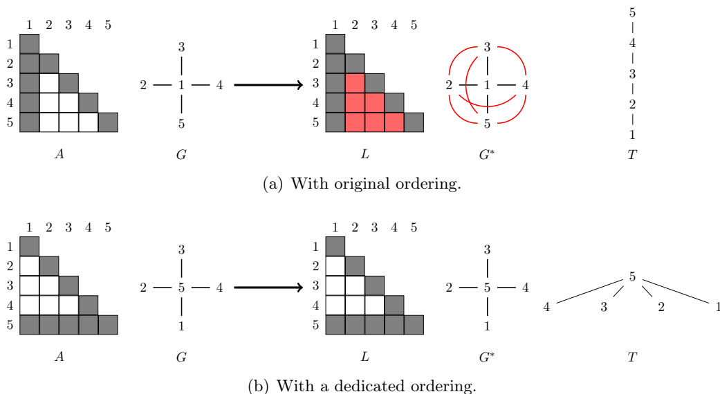
Figure 1.1: Two different orderings for a five unknowns system. The original sparse matrix is A , associated with its graph G . The factorized matrix is L and in G^* fill-in edges were added. The elimination tree T gives dependencies between unknowns elimination.
