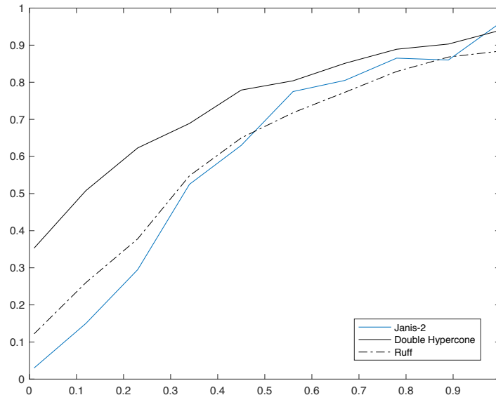
Figure 12.1: \mathbb{P}_{fn} as a function of \sigma_Z^2 for \mathbb{P}_{fp} \leq \eta = 10^{-6} , n = 2048 , \sigma_X = 1 and P = 0.01 . Janis (order 2) vs. the double hypercone ( black line ) and the ruff detector \rho = 1/128 ( black dotted line ).
