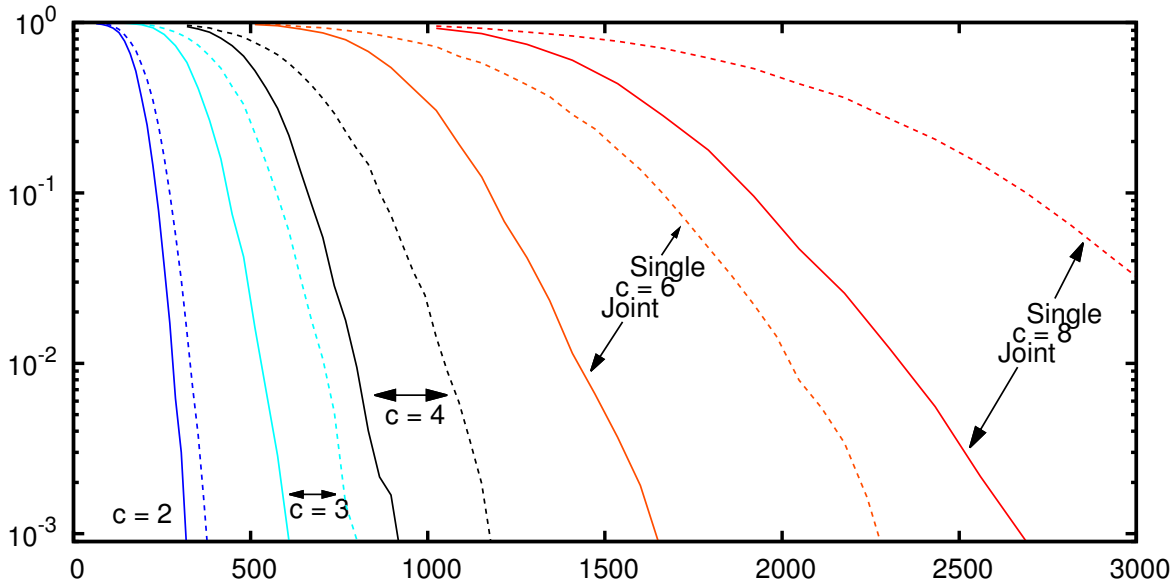
Figure 5.9: Code length vs. \mathbb{P}_e = \mathbb{P}_{\text{FP}} + \mathbb{P}_{\text{FN}} for n = 10^6 users and c colluders performing worst-case attack against a single decoder; c_{\text{max}} = 8 . This experiment generated 10^{10} codewords.
