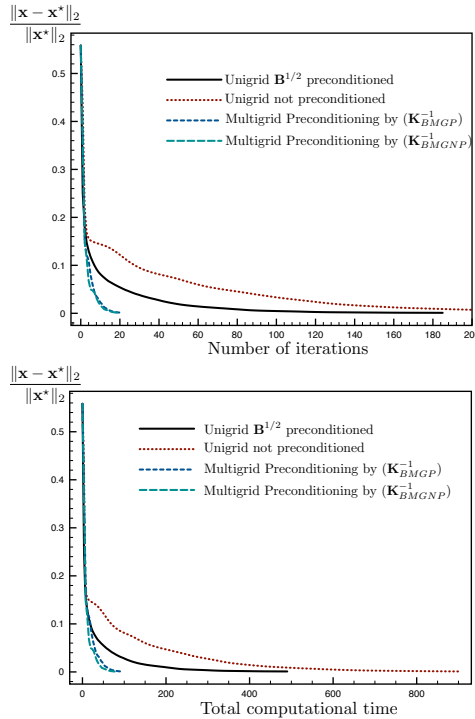
Figure 4.4: Refinement factor \rho = 3 . Evolution of the error \left( \frac{\|\mathbf{x} - \mathbf{x}^*\|_2}{\|\mathbf{x}^*\|_2} \right) as a function of the number of fine grid iterations (top) and of the total computational time in seconds (bottom) for L_{\text{corr}}/\Delta x = 10 and with three grid levels.
