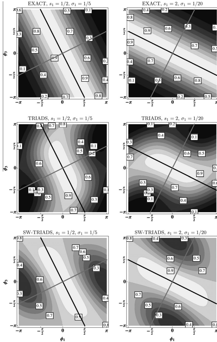
Fig. 4. Exact amplification factor in the (\phi_1, \phi_3) plane for s_1 = 1/4(1 + s_1^2) (i.e., when the (EXP) scheme is stable) with s_1 = 1/2 (top, left) and s_1 = 2 (top, right) in the two-dimensional (x_1, x_3) case (i.e., \kappa_2 = 0 ). Amplification factor for the (EXP) scheme with the TRIADS discretization (middle, left for s_1 = 1/2 and middle, right for s_1 = 2 ) and with the SW-TRIADS discretization (bottom, left for s_1 = 1/2 and bottom, right for s_1 = 2 ) for the same values of \sigma_1 . The thick black line is D_1 = 0 , the thick gray line is D_2 = 0 .
