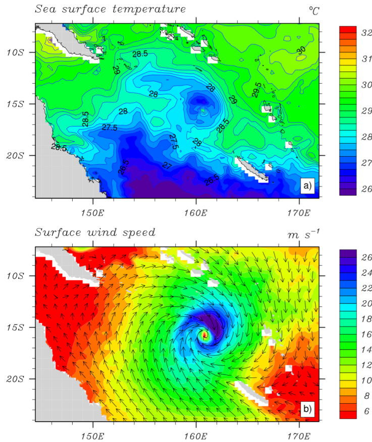
Figure 2.6: Snapshots (March 12, 2003 at 8 p.m. GMT) of (a) ROMS sea surface temperature (b) WRF 10 meter winds during a coupled simulation.
