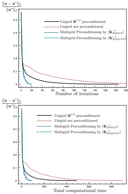
Figure 12. Refinement factor \rho = 3 . Evolution of the error \left(\frac{\|x - x^*\|_2}{\|x^*\|_2}\right) as a function of the number of fine grid iterations (top) and of the total computational time in seconds (bottom) for L_{\text{corr}}/\Delta x = 10 and with three grid levels.
