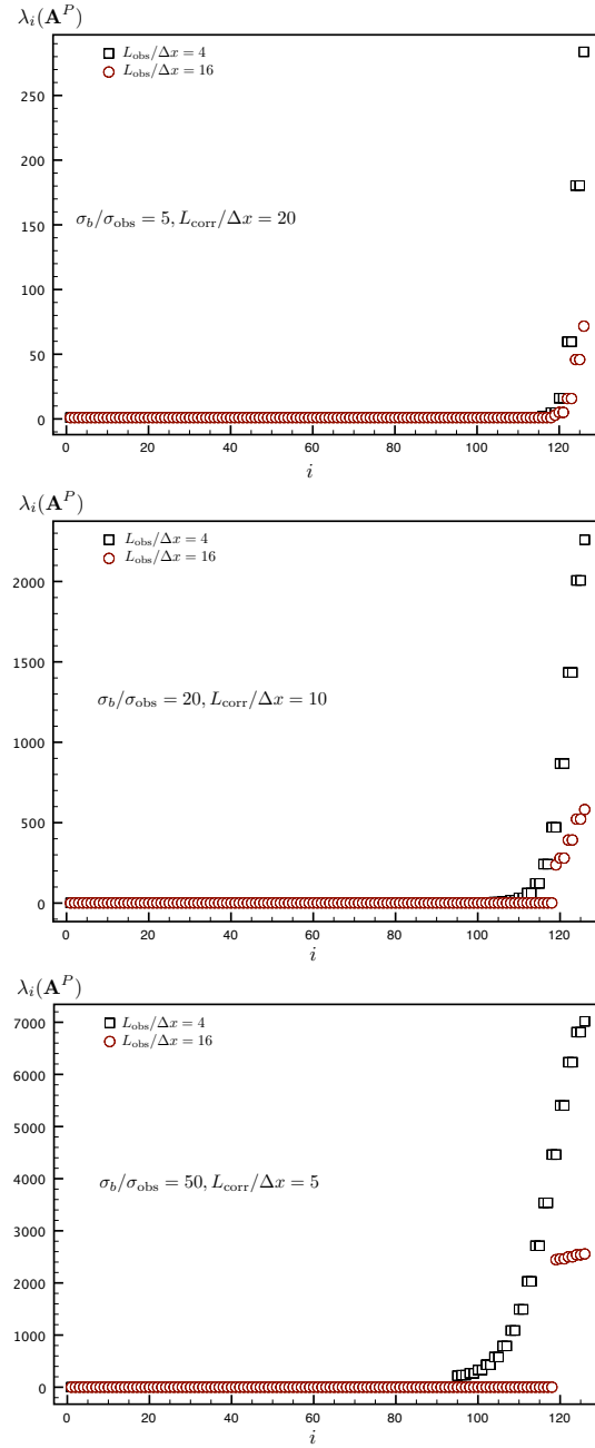
Figure 2. Eigenvalue spectrum ( \lambda_i(\mathbf{A}^P), i = 1 \dots N ) of the preconditioned version for the 1DVAR case ( N_{\text{obs}} = 1 ) and for \sigma_b/\sigma_{\text{obs}} = 5, L_{\text{corr}}/\Delta x = 20 (top), \sigma_b/\sigma_{\text{obs}} = 20, L_{\text{corr}}/\Delta x = 10 (middle) and \sigma_b/\sigma_{\text{obs}} = 50, L_{\text{corr}}/\Delta x = 5 (bottom)
