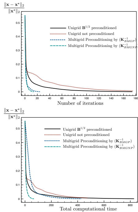
Figure 11. Refinement factor \rho = 2 . Evolution of the error \left(\frac{\|\mathbf{x} - \mathbf{x}^*\|_2}{\|\mathbf{x}^*\|_2}\right) as a function of the number of fine grid iterations (top) and of the total computational time in seconds (bottom) for L_{\text{corr}}/\Delta x = 10 and with three grid levels.
