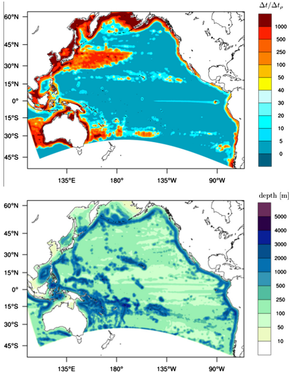
Fig. 10. Annual mean of the maximum value of the ratio \Delta t / \Delta t_p for each water column (top), with \Delta t the time-step of the ROMS model using the (MSC) scheme to advance the rotated biharmonic operator and \Delta t_p the time-step which would be needed to advance the same operator but with the (EXP) scheme. Depth of the maximum (bottom). \Delta t / \Delta t_p is first computed using seasonal averages and is then averaged to get the annual mean.
