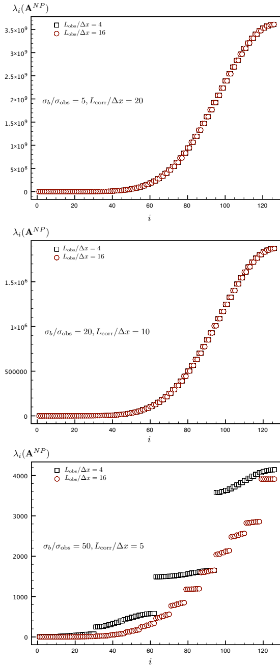
Figure 1. Eigenvalue spectrum ( \lambda_i(\mathbf{A}^{NP}), i = 1 \dots N ) of the non-preconditioned version for the 1DVAR case ( N_{\text{obs}} = 1 ) and for \sigma_b/\sigma_{\text{obs}} = 5, L_{\text{corr}}/\Delta x = 20 (top), \sigma_b/\sigma_{\text{obs}} = 20, L_{\text{corr}}/\Delta x = 10 (middle) and \sigma_b/\sigma_{\text{obs}} = 50, L_{\text{corr}}/\Delta x = 5 (bottom)
