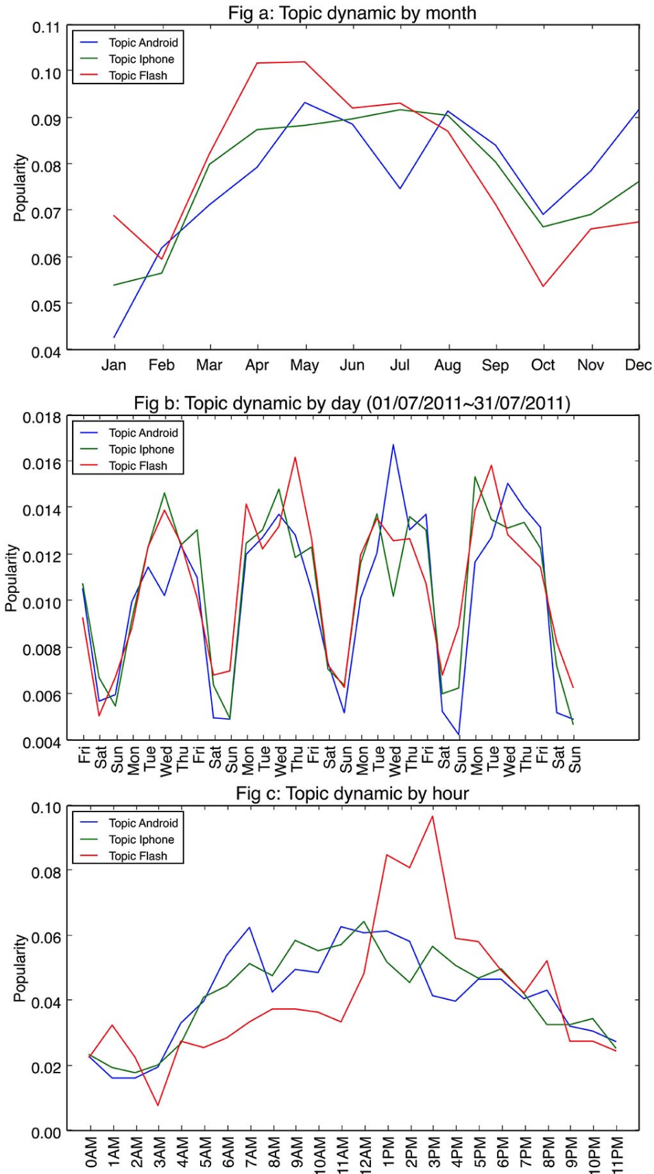
Figure 7.4: Topic dynamics
