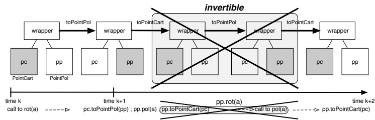
FIGURE 8.2 : Conversion inversible
