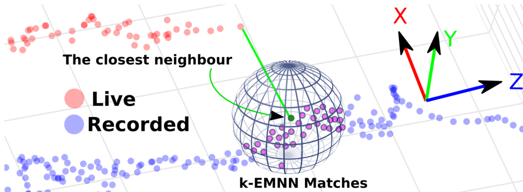
Figure 7.3: k -Nearest neighbour electromagnetic tracker matches. Firstly, the EMNN is obtained using the 3D position match. Then within a radius r around this match, all the points on the trajectory are considered as the k -EMNN matches.
