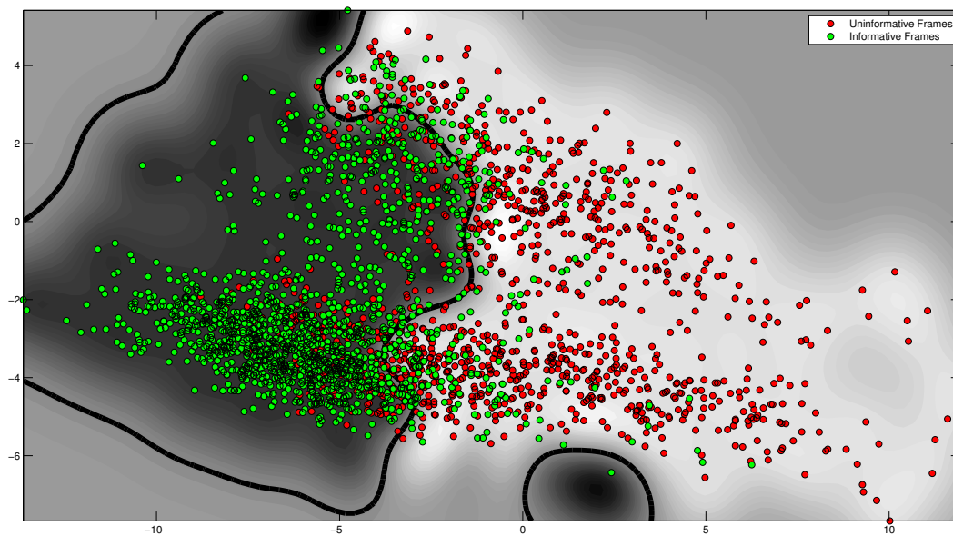
Figure 7.6: 2D Decision Boundary WL, using \kappa = 2 principal components.
