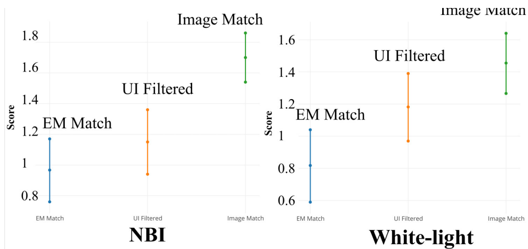
Figure 7.12: This figure shows the comparison between confidence intervals for the average scores for matches obtained using EM based approach, UI filtered EM match and the best performing descriptor (mLBP, mLIOP) for constrained image match.
