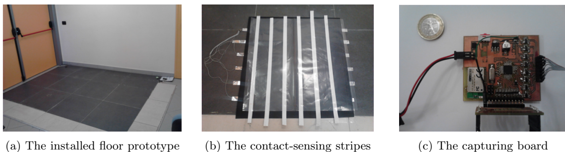
Figure 2.21 – The sensing floor presented by Lombardi et al. in [85].
