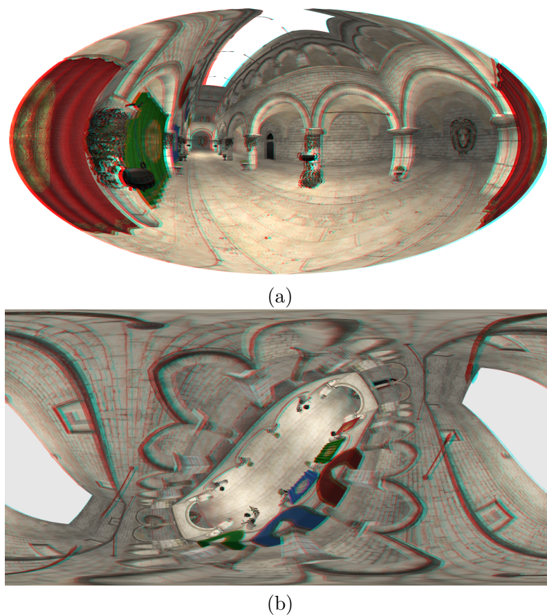
Figure 5.6 – Stereoscopic (anaglyph for reader convenience) rendering of 360° view using (a) a Hammer projection and (b) an equirectangular projection. The images are computed at real-time framerate.
