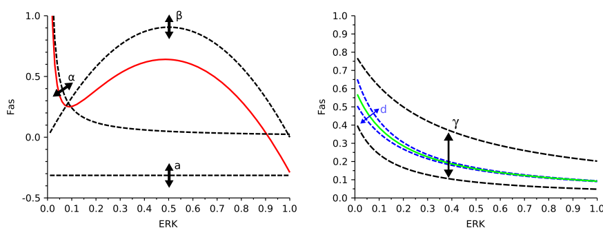
Fig. 1. Null-clines f and g defined in (3) and (4). Left panel: the f null-cline (solid red line) and the impact of parameters of Eq. (1). Right panel: the g null-cline (solid green line) and the impact of parameters of Eq. (2). (For interpretation of the references to color in this figure legend, the reader is referred to the web version of this article.)
