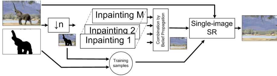
Figure 8.2: The framework of the proposed method.
