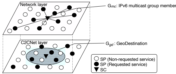
Fig. 6. Propagation of multicast SrvRqst packets.
