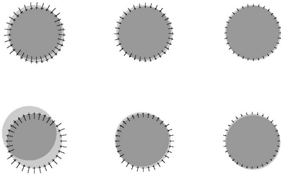
Figure 6. Next three iterations (top row, attractive points; bottom row, demons).
