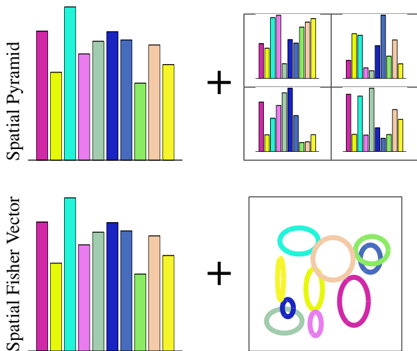
Figure 1. The spatial pyramid image representation concatenates visual word histograms of the complete image and spatial cells. Our spatial Fisher vector representation models spatial layout by the mean and variance of the occurrences of each visual word.
