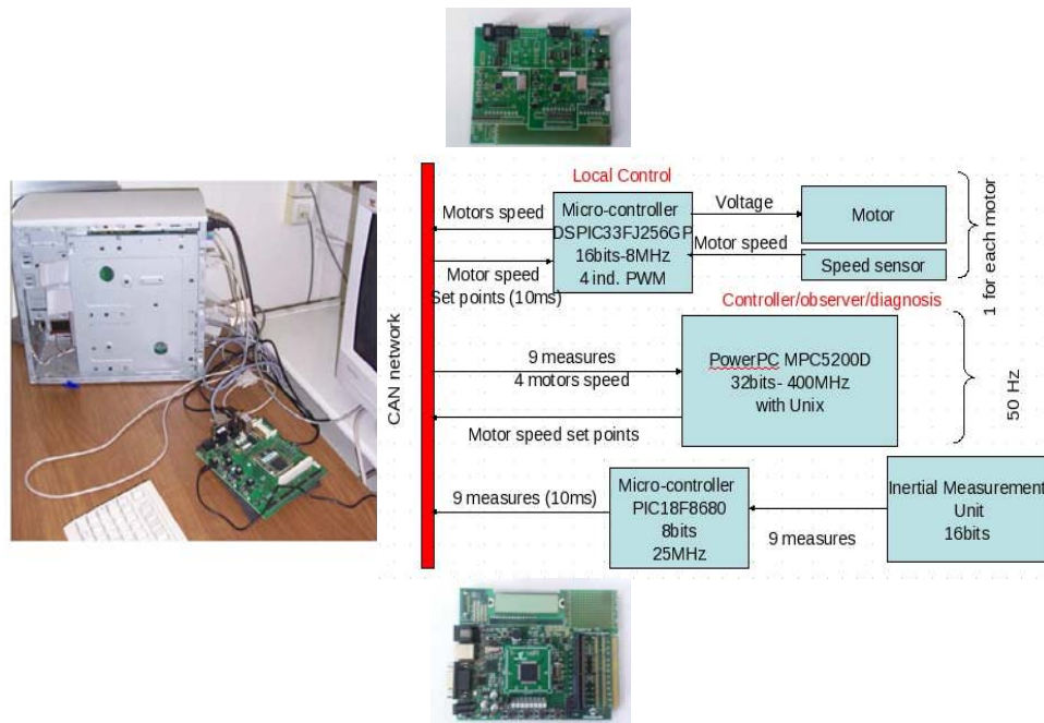
Figure 2: Real hardware.
