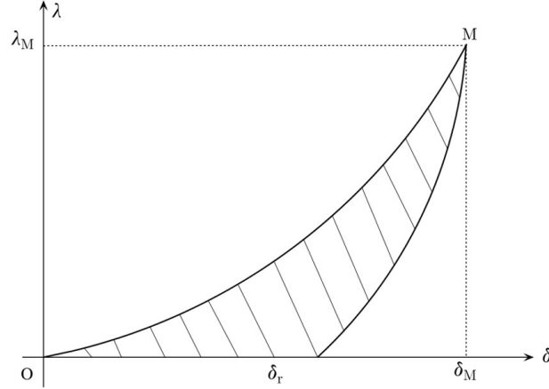
Figure 1: Bi-stiffness contact compliant model.
