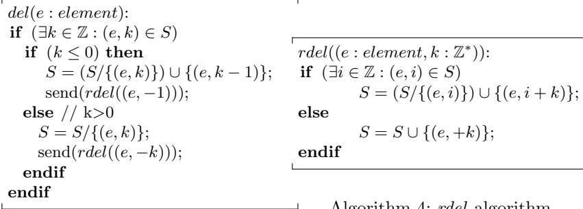
Algorithm 4: rdel algorithm
