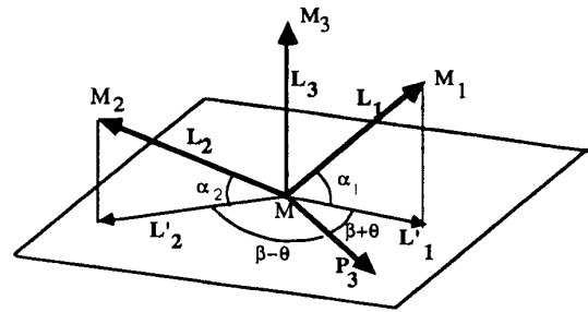
Figure 4: An "object frame" is associated with the four points.
