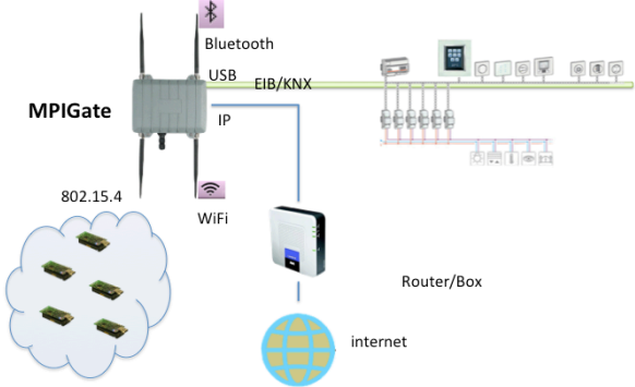
Figure 1. MPIGate in an assisted living network.
