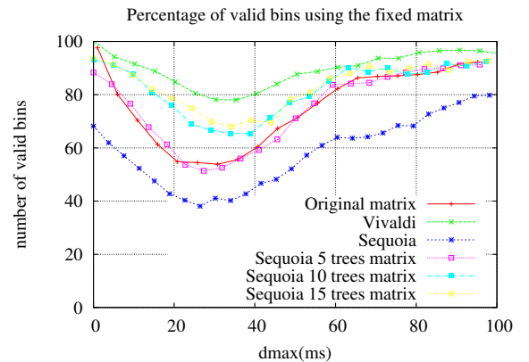
Figure 4. Percentage of valid bins for BPDC, for different values of d_{\max} , using different embeddings, using the fixed latency matrix.
