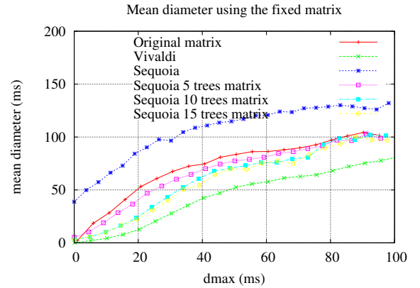
Figure 3. Mean diameter of built bins for BPDC, for different values of d_{\max} , using different embeddings, using the fixed latency matrix.
