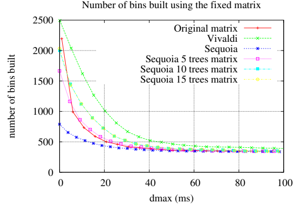
Figure 2. Number of built bins for BPDC, for different values of d_{\max} , using different embeddings, using the fixed latency matrix.
