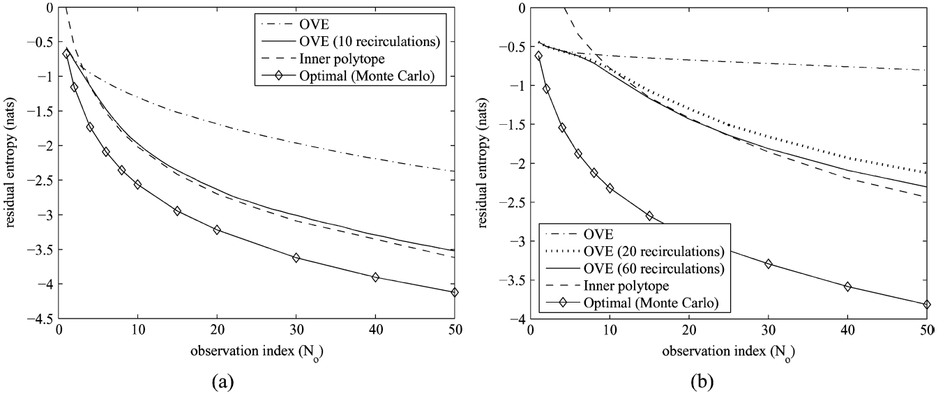
Fig. 6. Performance comparison (in terms of residual entropy) for the hexagonal lattice (a) and Gosset lattice E_8 (b), for KMA and \alpha = 0.5 .
