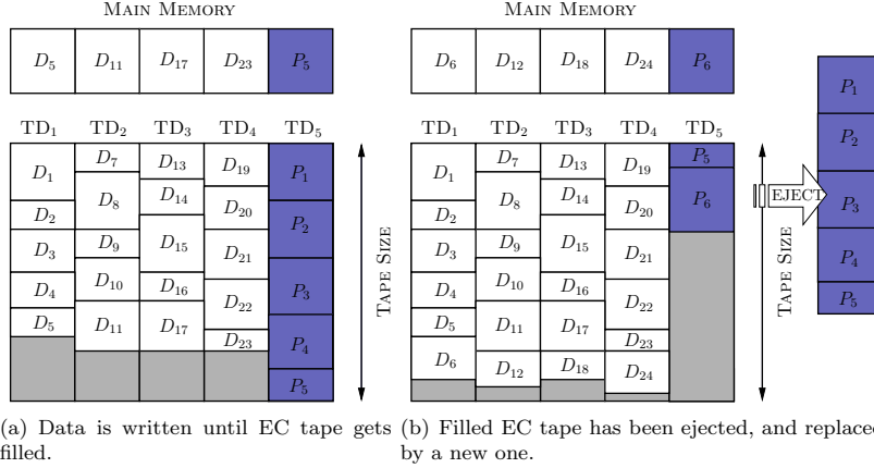
Figure 2: Writing data with PARALLEL policy with X = 4 and Y = 1 .
