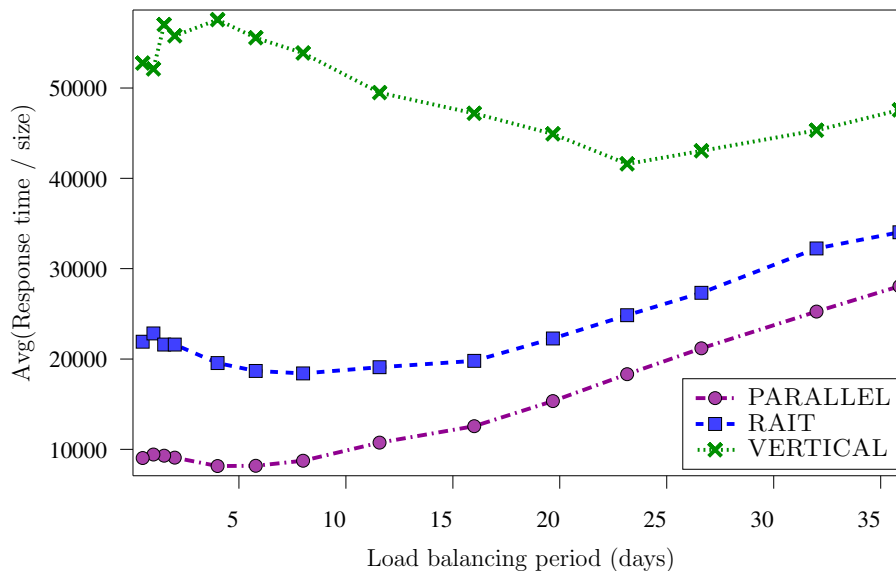
Figure 10: Impact of LOAD-BALANCER period on performance.
