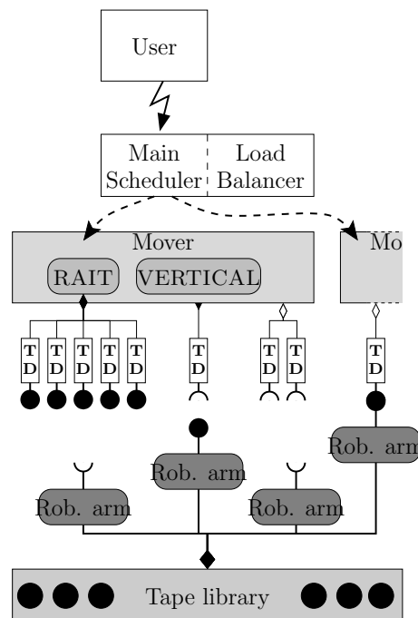
Figure 4: Model of the simulated platform
