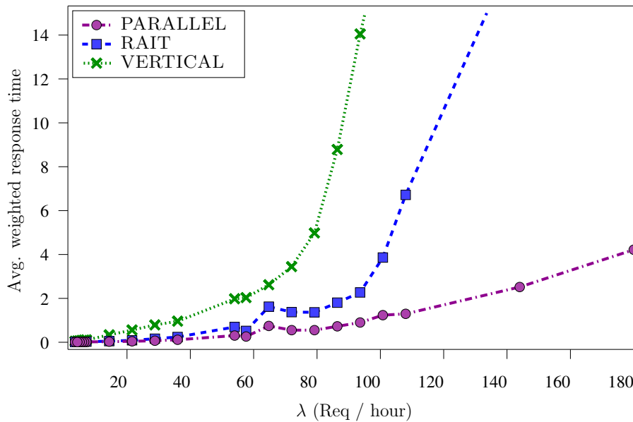
Figure 7: Impact of arrival rates on the average weighted response time for medium-size files ( B = 256 MB for RAIT).
