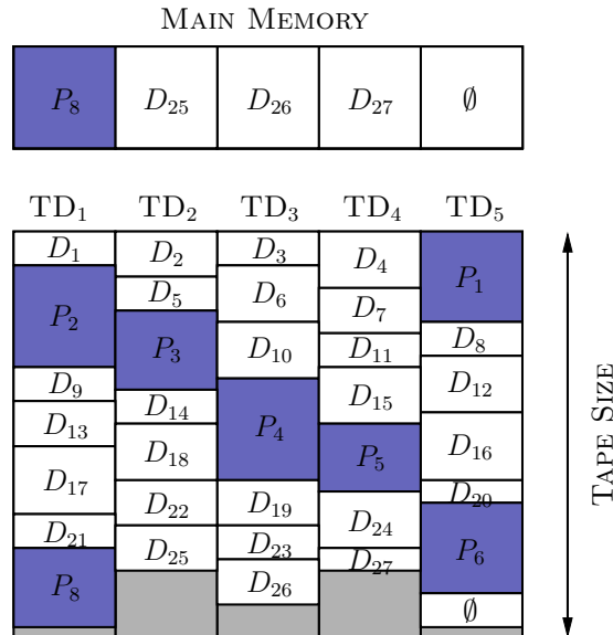
Figure 1: Writing data with RAIT policy for X = 4 and Y = 1 .
