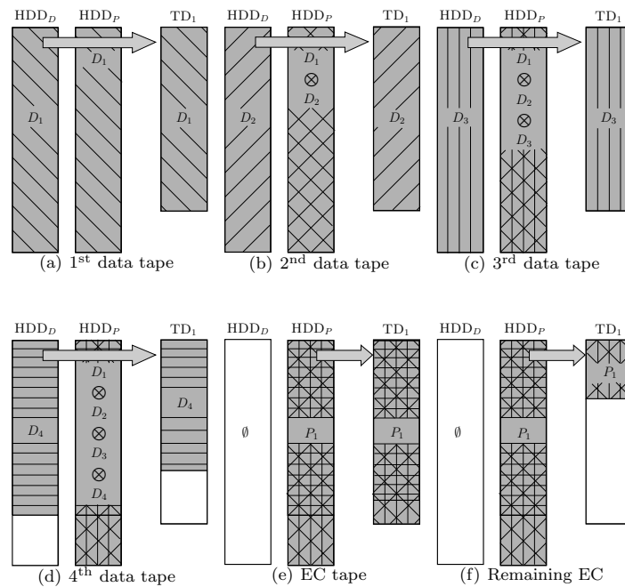
Figure 3: Writing data with VERTICAL policy with X = 4 and Y = 1 .
