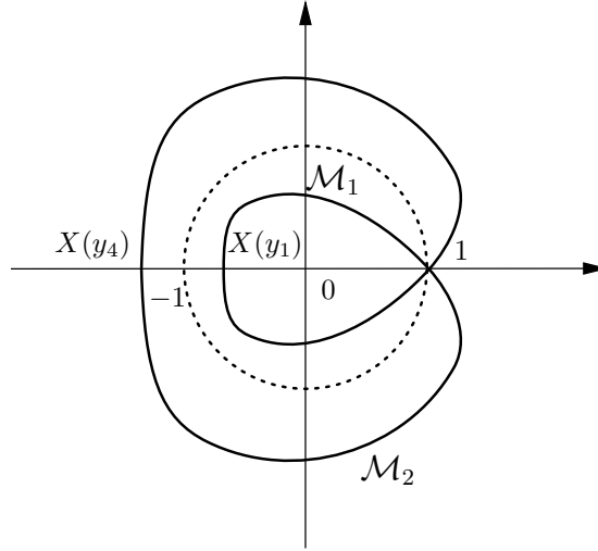
Fig. 2.1: The contour \mathcal{M}_1 \cup \mathcal{M}_2 for R < 0
