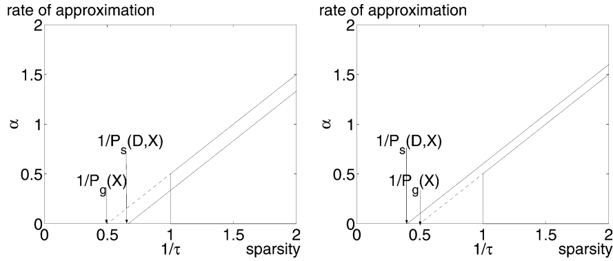
FIGURE 2 Comparison of the thresholding-Jackson embedding line and the Chebyshev-Jackson one. The leftmost graph depicts a situation where the thresholding-Jackson embedding is valid for a larger range of values of 1/\tau than the Chebyshev-Jackson one, but the latter is stronger on its range of validity. The rightmost corresponds to the opposite situation, where the thresholding-Jackson embedding line is better than the Chebyshev-Jackson one throughout its domain of validity.
