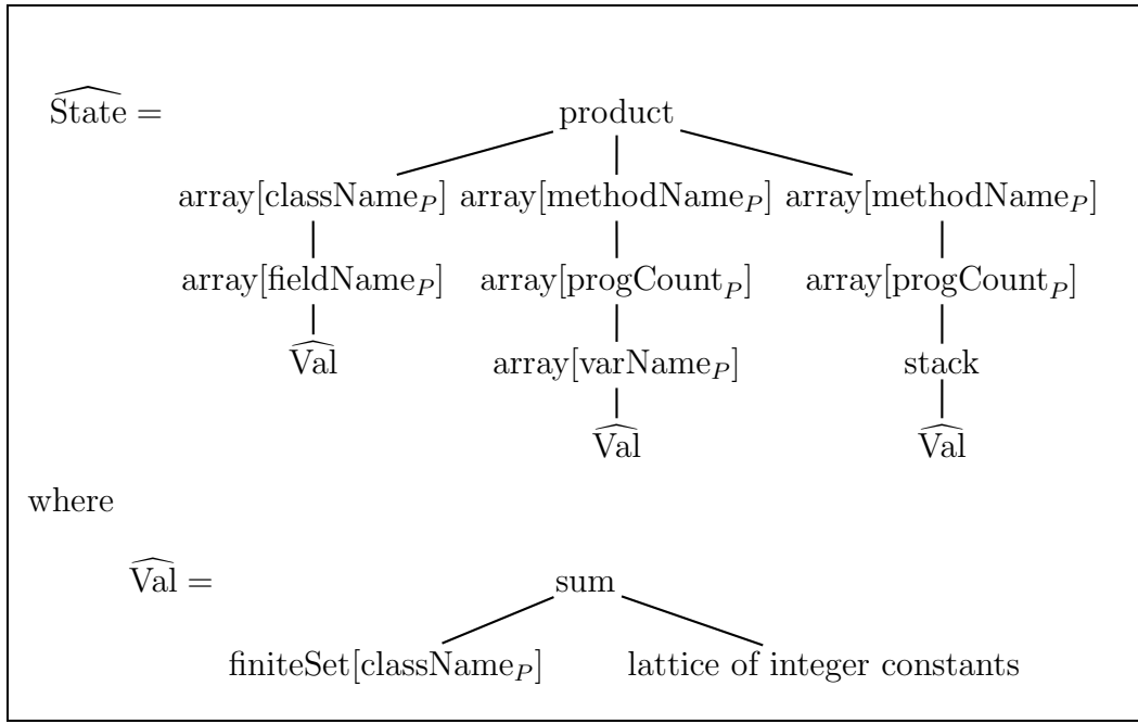
Fig. 2. The lattice of abstract states (each \text{xX}_P represents the number of distinct \text{xX} elements in program P ).
