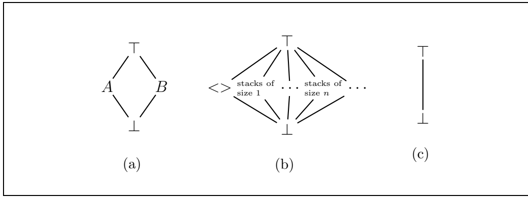
Fig. 1. Hasse diagrams of lattices
