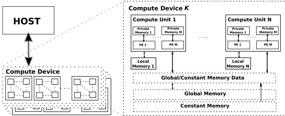
Figure 1: OpenCL Platform and Memory Model
