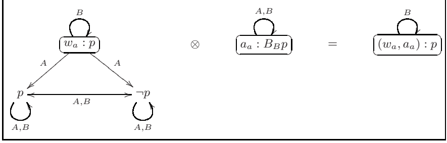
Fig. 3. Failure of seriality preservation
