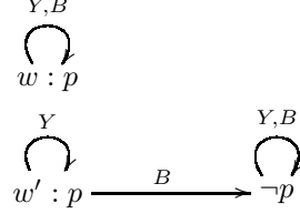
FIG. 7. Epistemic model (M, w) (above) and (M', w') (below)
