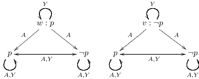
FIG. 3: An internal model : multi-agent possible world (M_1, w) (left) and multi-agent possible world (M_2, v) (right)
