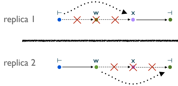
Figure 17: Monotonic DAG: remove is not live. Dashed: removed; dotted: added.
