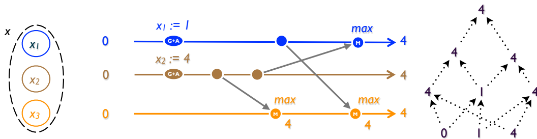
Figure 4: State-based replication
