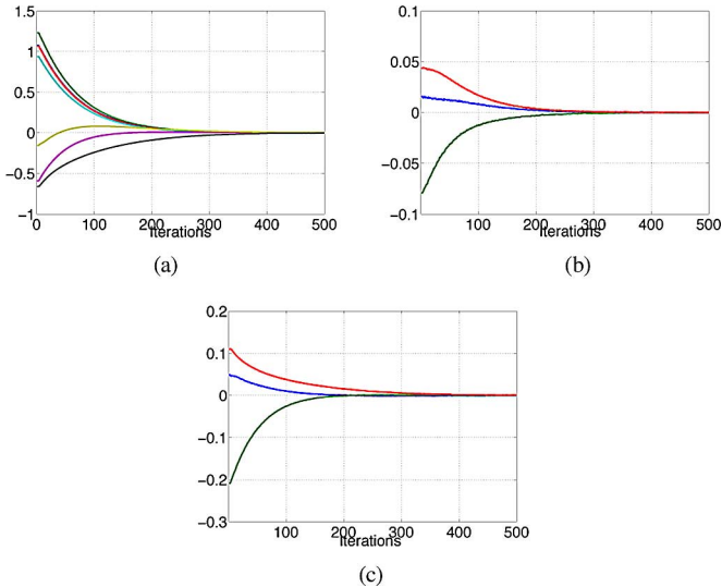
Fig. 19. Results for four coplanar points (i.e., generic motion using s_{\Delta} ). (a) Feature errors, (b) translational velocities (in meters per second), and (c) rotational velocities (in radians per second).
