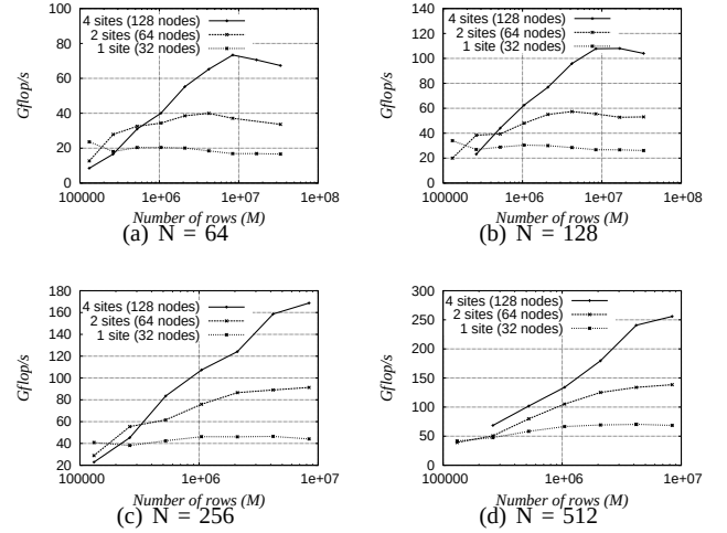
Fig. 4. TSQR Performance.
