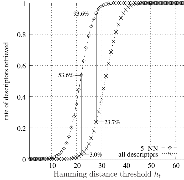
Fig. 5. HE: filtering effect on the descriptors within a cell and on the 5 NNs: trade-off between the rate of cell descriptors and the rate of NN that are retrieved for d_b = 64 .
