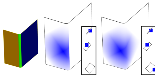
Figure 4: Matching texel colors across chart boundaries does not ensure continuity. Here, a texel lying on the brown chart propagates its value to the texel on the green chart, but cannot reach the blue chart (middle). Our texel class approach resolve such problems (right).
