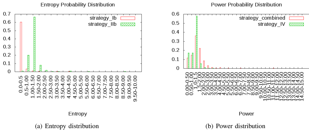
Fig. 2. Probability distribution
