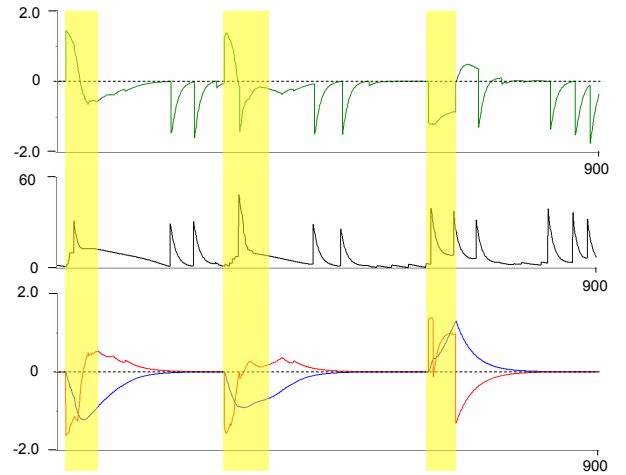
Fig. 6. Evolution of relevant variables during navigation in scenario C: \omega (green, in \text{rad s}^{-1} ), image error e (black, in pixels), \varphi (blue, in rad) and \dot{\varphi} (red, in \text{rad s}^{-1} ). The iterations with non-null H are highlighted in yellow.
