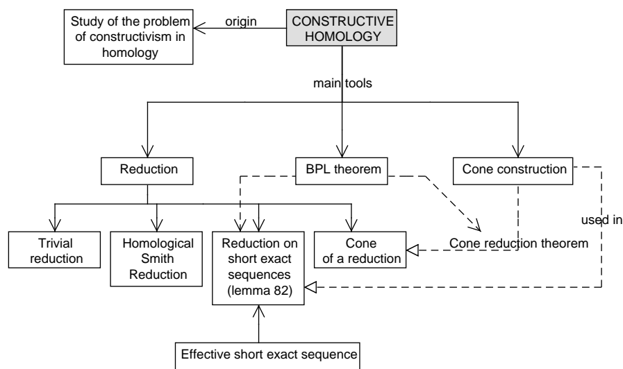
Figure 3.1: Diagram of concepts of Constructive Homology. The BPL theorem (Basic Perturbation Lemma) is the key result to prove the Cone Reduction Theorem and Lemma 82.
