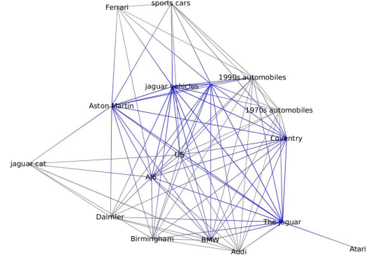
Figure 4. Min_{50} -DIS for the Jaguar example
