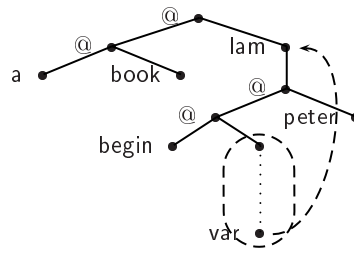
Figure 5. Relaxed semantic representation of (1)
