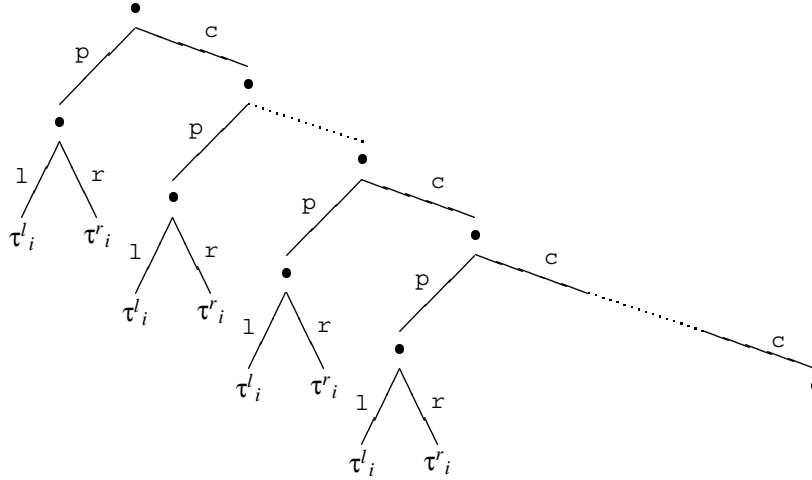
Fig. 4: The value of x' in the formula \text{select}(y_l, y_r, x) where x is as in Figure 3.
