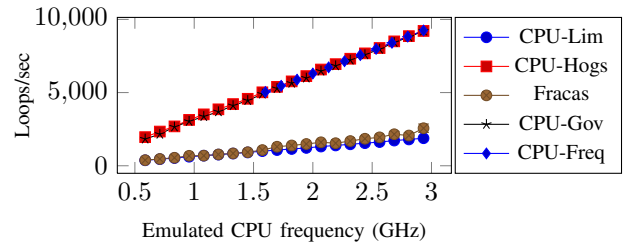
(f) Multithreading on 8 cores
