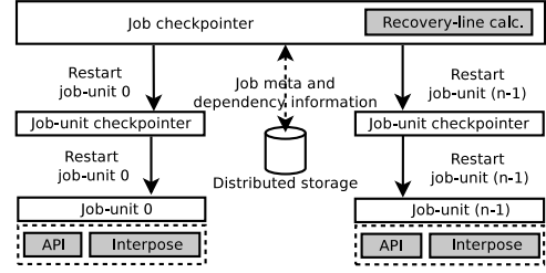
Fig. 7. Application recovery - Permanent failure
