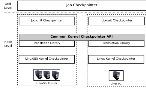
Fig. 1. XtreamOS Grid-Checkpointing Architecture [9]
