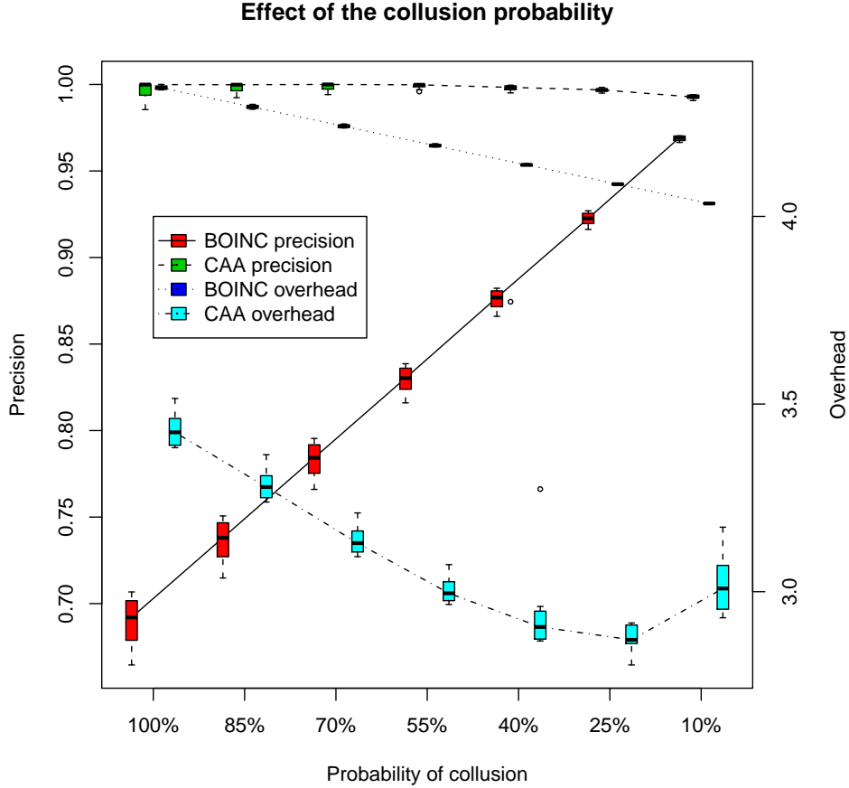
Figure 5: Performance of two methods with 2,000 workers, fully reliable plus one colluding group with 800 workers and varying collusion probability.
