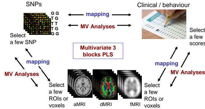
Fig. 2. The data available and how to combine them in mapping studies (one to many) or through multivariate PLS (many to many). Three PLS block can be used to integrate these data. Mappings and multivariate techniques often require variable selection or regularization because of the N \ll P problem.
