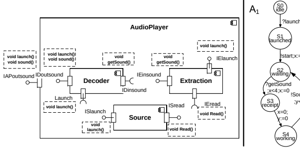
Figure 2. Example of an audio player component
