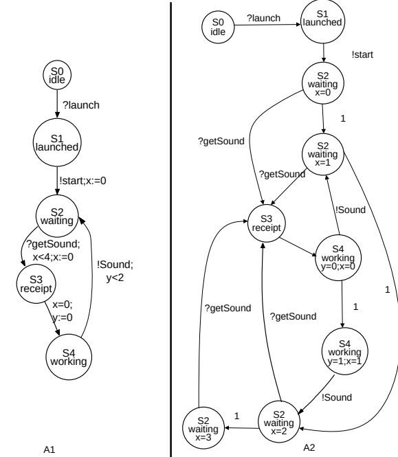
Figure 4. Transformation of automata
