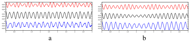
Figure 4: Multiresolution test: vertical position of an oscillating cube over time, using mass-springs (a) or Cauchy FE (b). The cube is sampled at different resolutions, using 27 nodes (red), 57 nodes (black) or 135 nodes (blue). Note that the behavior changes undeniably as the level of detail changes.
